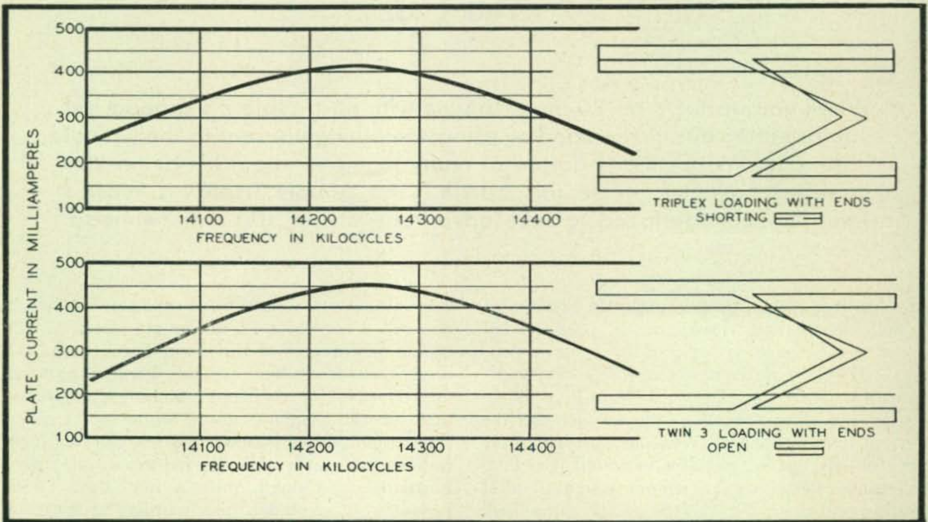
Fig. 2. Comparative final tank loading of the Triplex beam with the dipole end open and shorting. Although loading is somewhat better with the dipole ends open, constructional facilities favor closing the ends.
